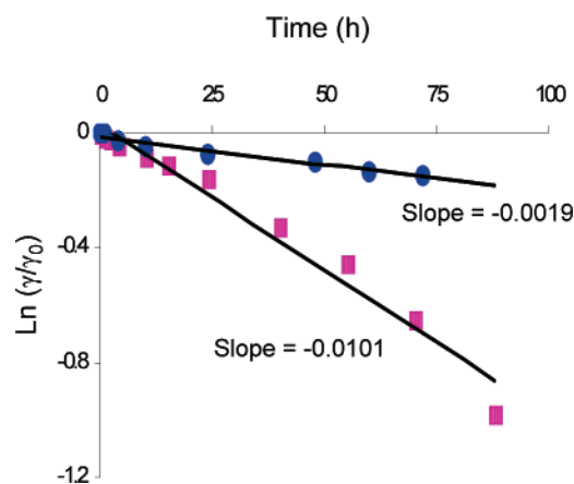
Figure 5. Hydrolysis kinetics at polymer C at pH 5.0 (■) and pH 7.4 (●).
