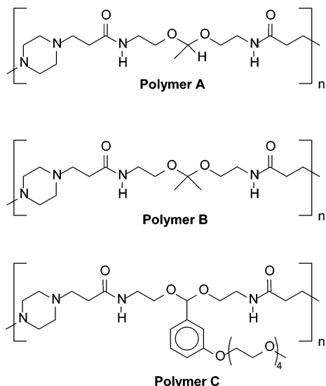
Figure 1. Acid-degradable poly(amidoamine)s.
